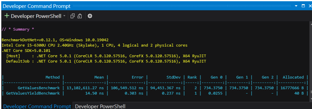
Figure 6.8 – The BenchmarkDotNet summary report showing the performance benefits of using the yield keyword
