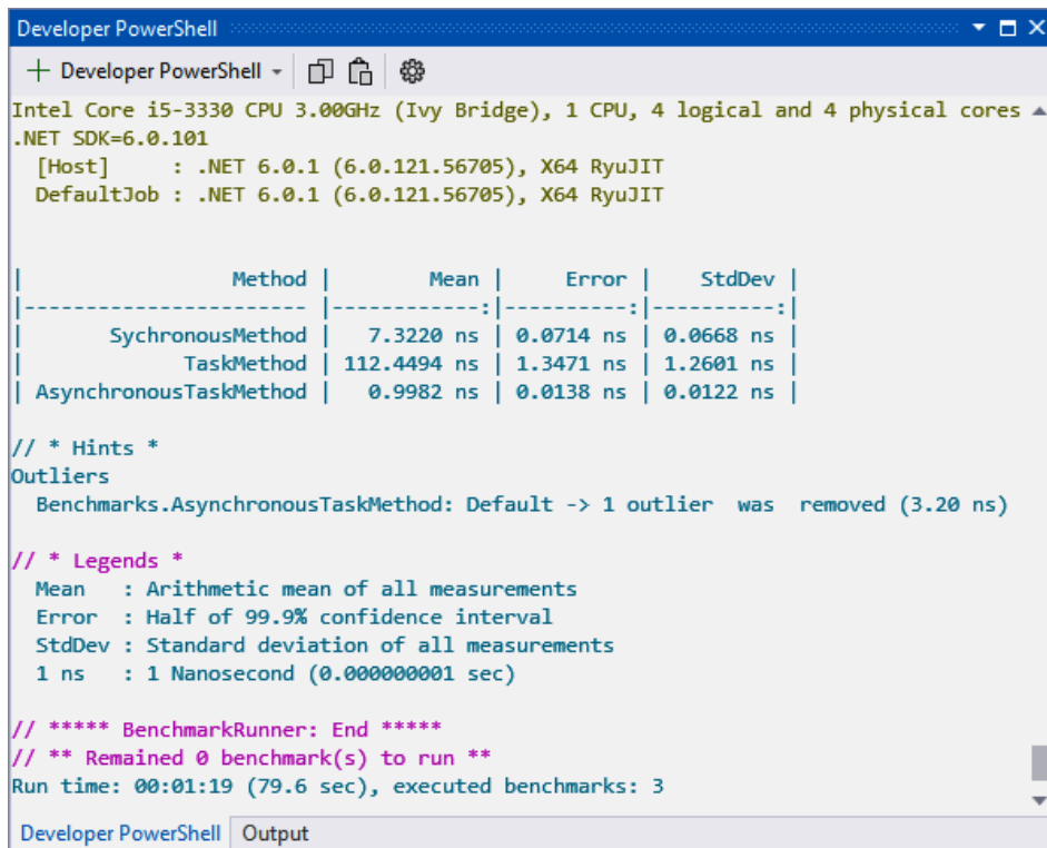
Figure 16.1 – The BenchmarkDotNet report for our CH16_AsyncronousProgramming Project
