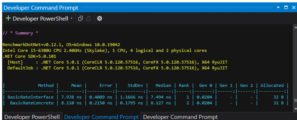
Figure 6.3 – The BenchmarkDotNet summary report showing the time difference between assigning IList<T> and List<T>
