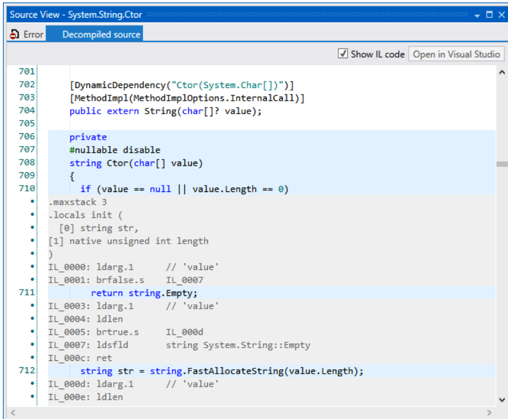
Figure 5.46 – The dotTrace Source View screen showing decompiled C# and IL source code
