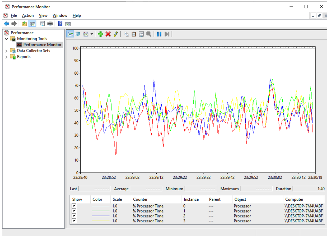
Figure 15.2 – Performance Monitor showing all our processors being used by our modified program
