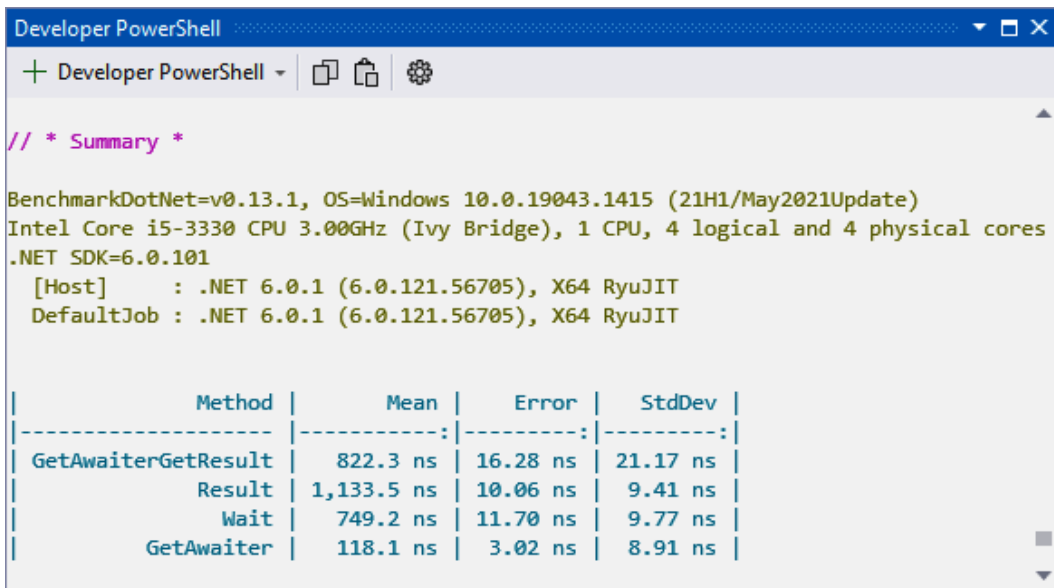
Figure 16.2 – The BenchmarkDotNet summary report for this section's methods
