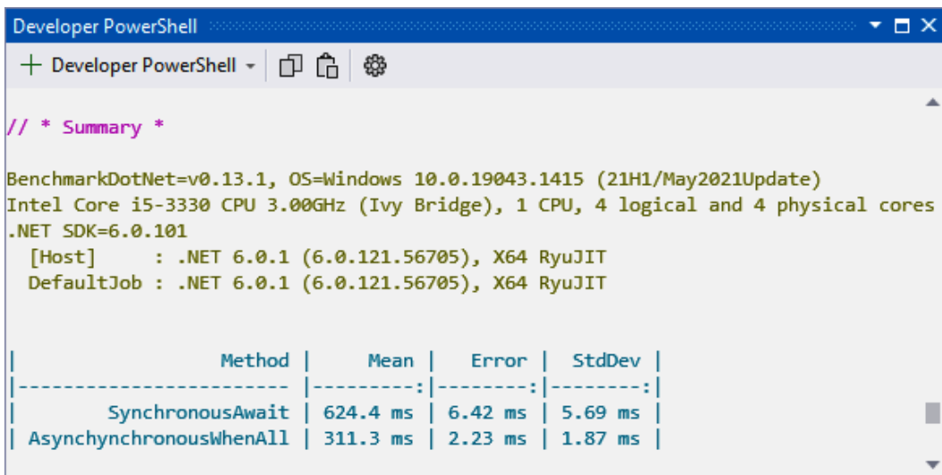
Figure 16.3 – The results of synchronous and asynchronous execution of multiple asynchronous calls
