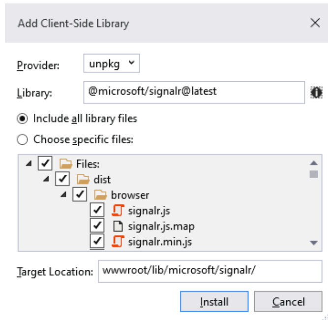
Figure 12.8 – The Add Client-Side Library configured to install SignalR
