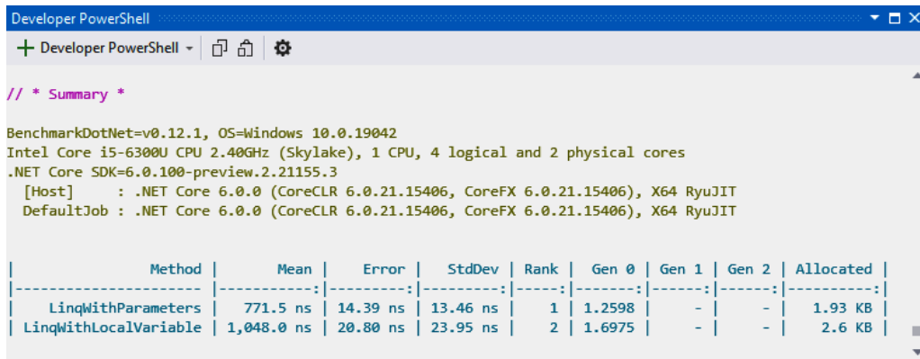
Figure 7.11: Closure benchmarks with and without parameters
