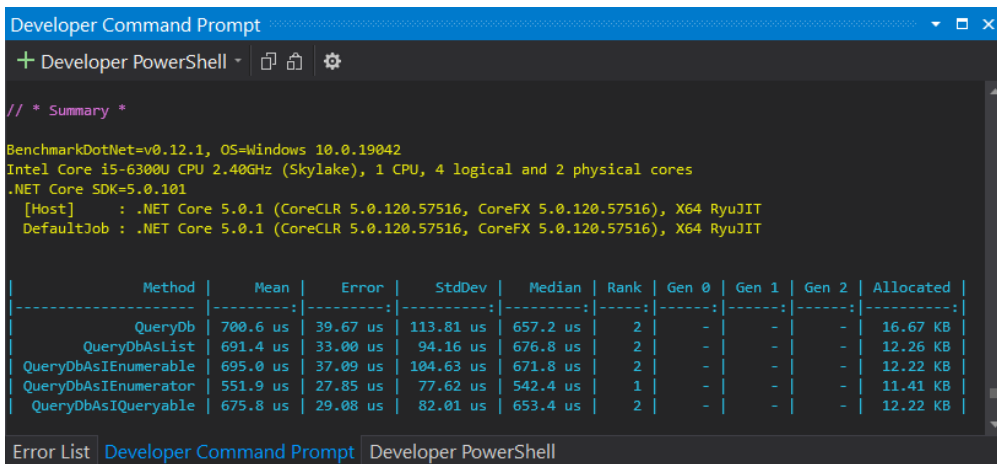
Figure 7.4: The different times and memory allocation of various database query types using LINQ
