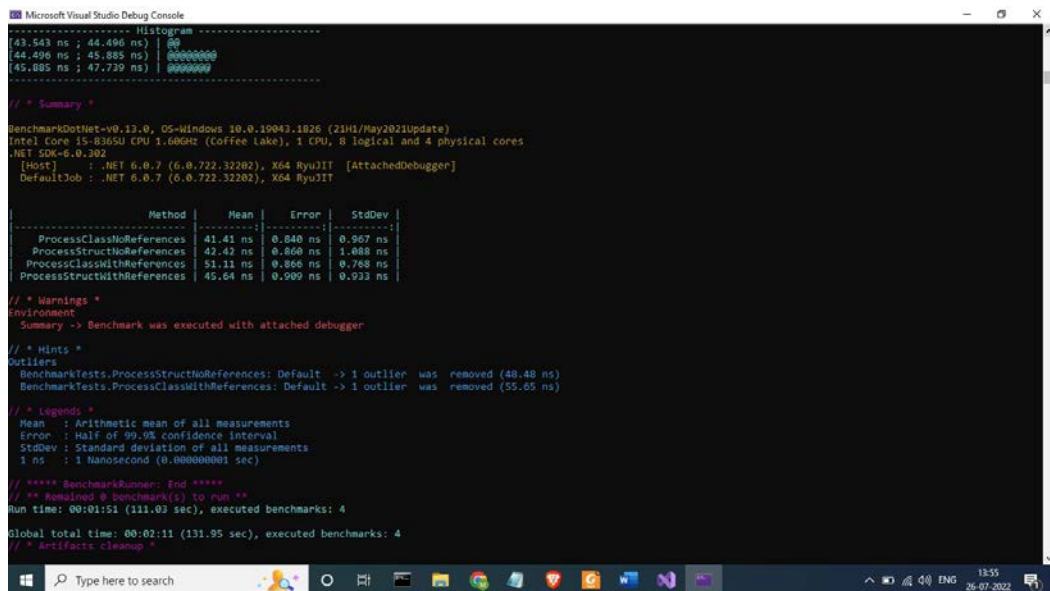
Figure 3.7 – The benchmark report comparing structs and classes with and without references
