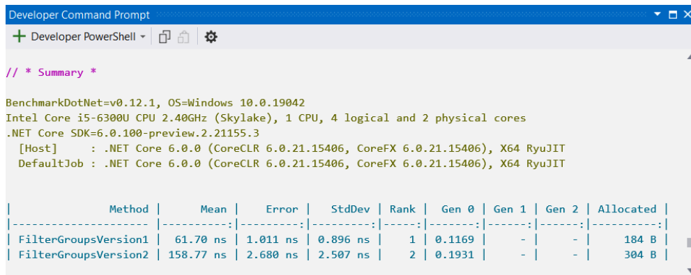
Figure 7.8: Benchmark Report for LINQ with and without using the let keyword
