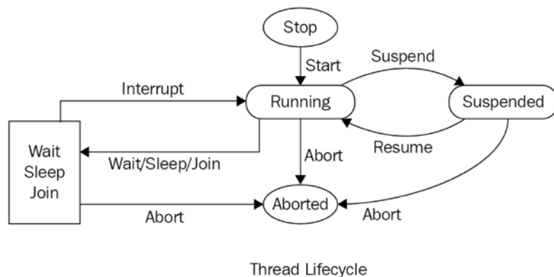
Figure 14.1 – The thread life cycle
