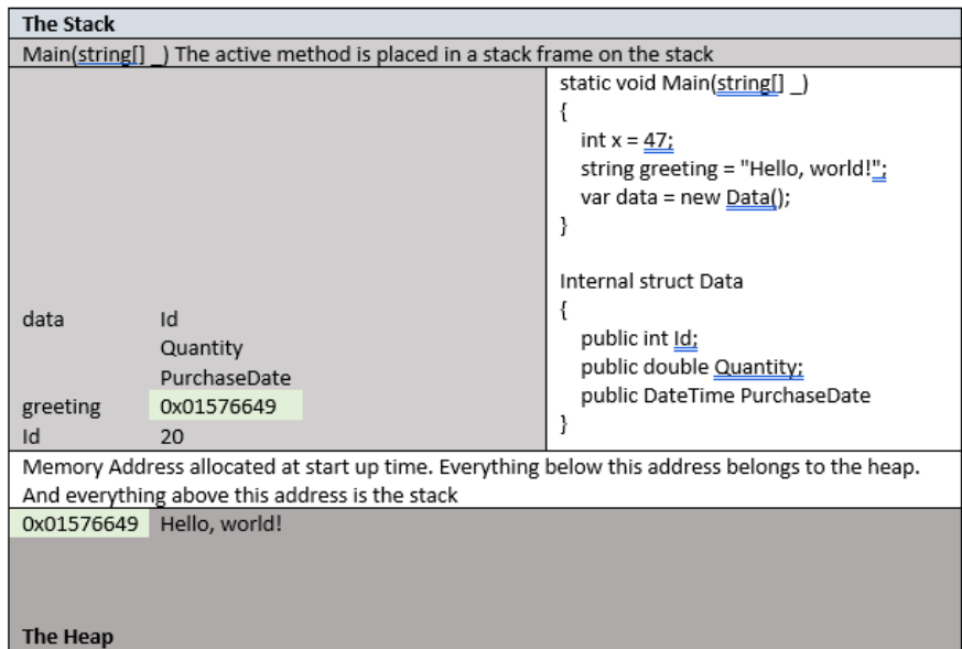
Figure 3.5 – The stack and heap at work
