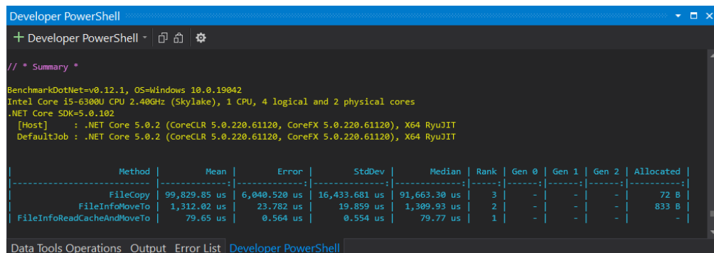
Figure 7.1 – The BenchmarkDotNet summary report for various file move operations
