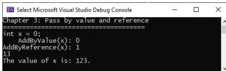
Figure 3.9 – Our integer has been updated inside the method we passed it into
